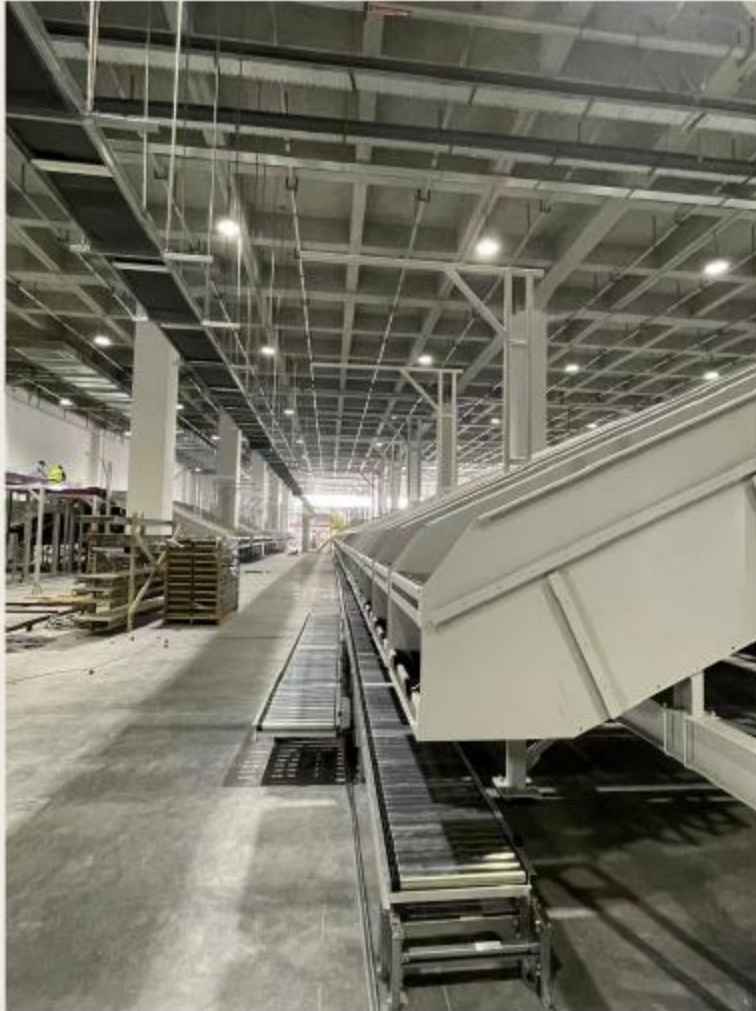
Puma Taicang—— Double layer chute production and site installation.
